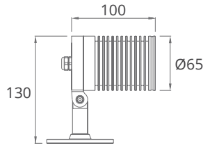
DC Version
