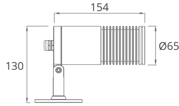
AC Version
